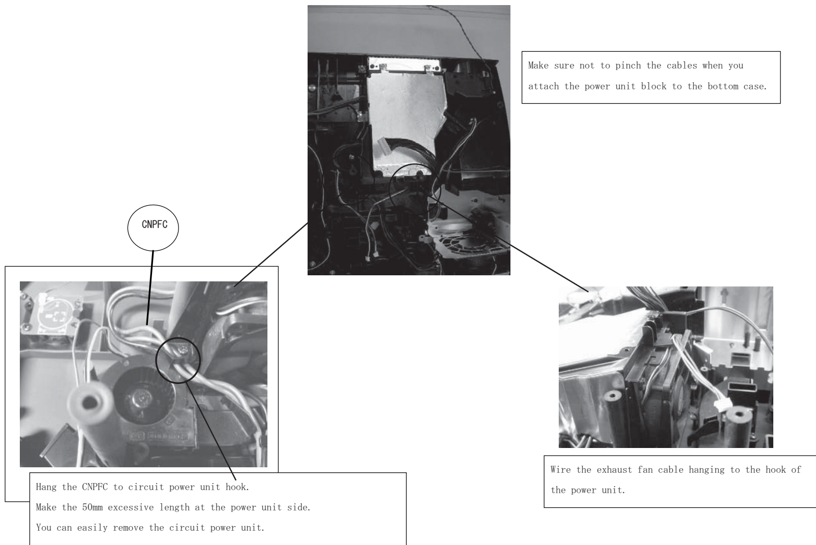
Wiring diagram 8
