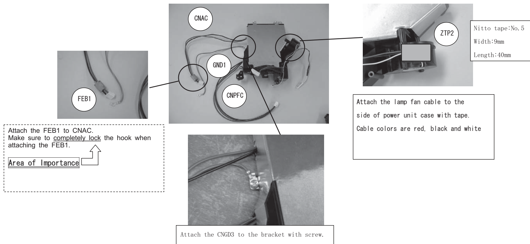
Wiring diagram 2
