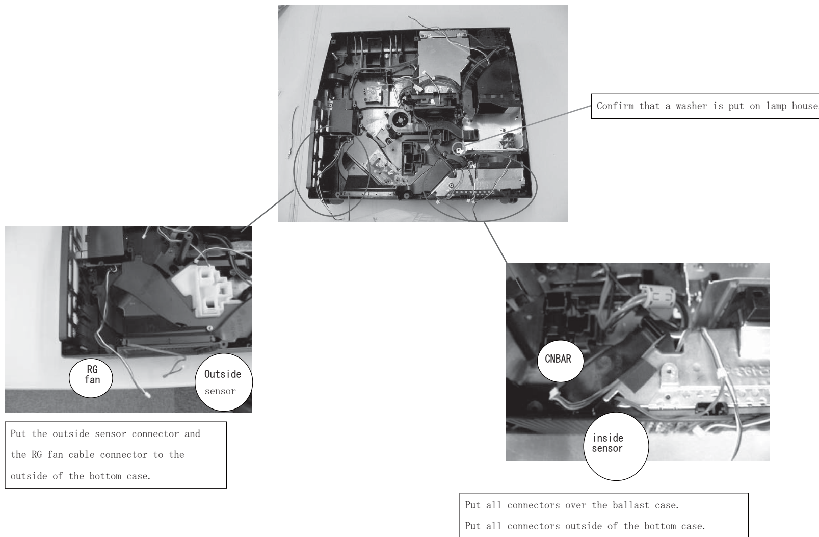
Wiring diagram 11
