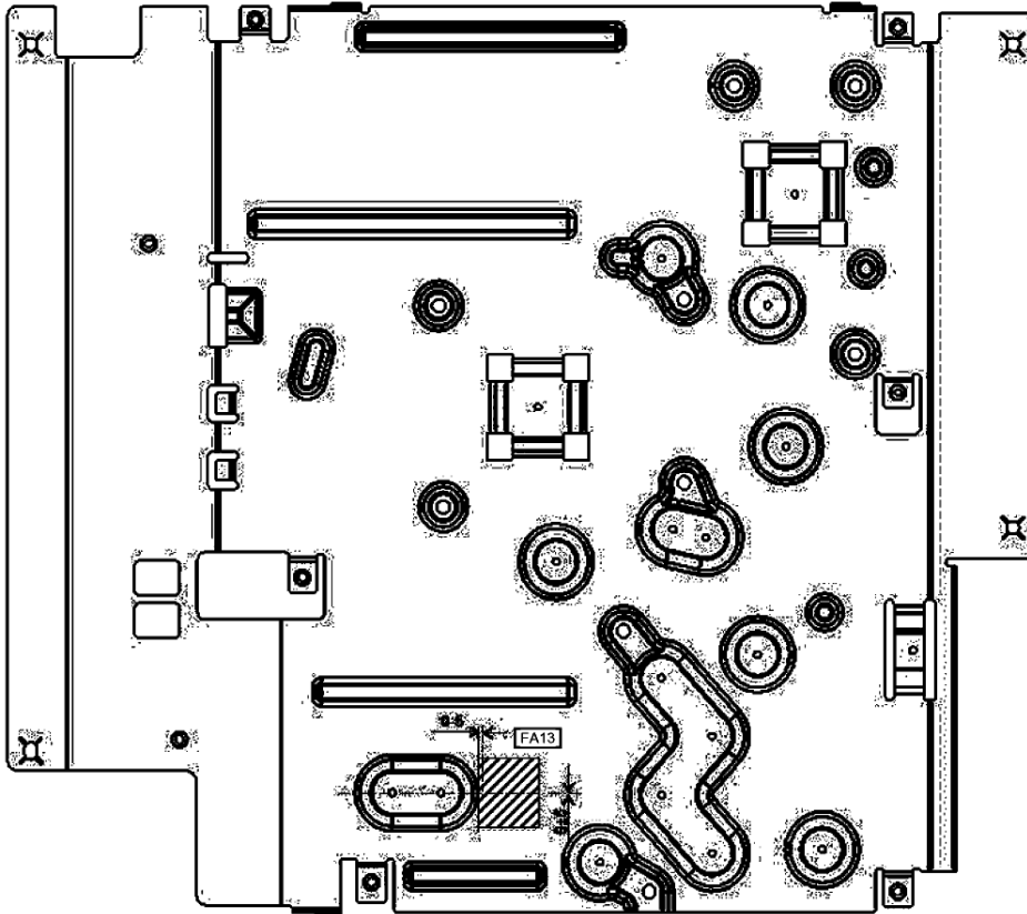
Heatsink A-REAR
