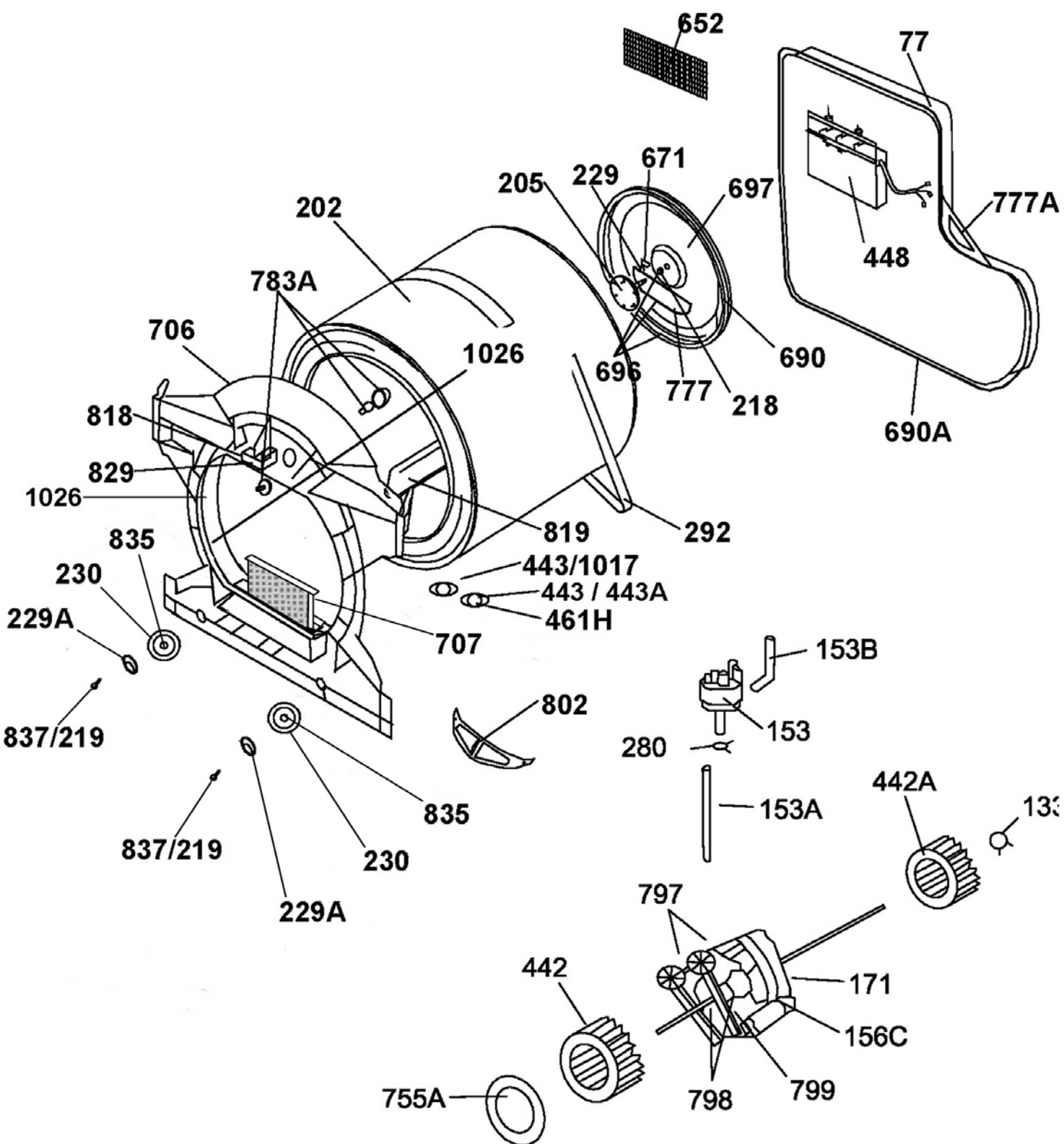
DRUM ASSY - CONDENSER
