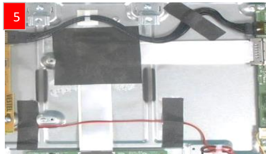
LVDS Cable
