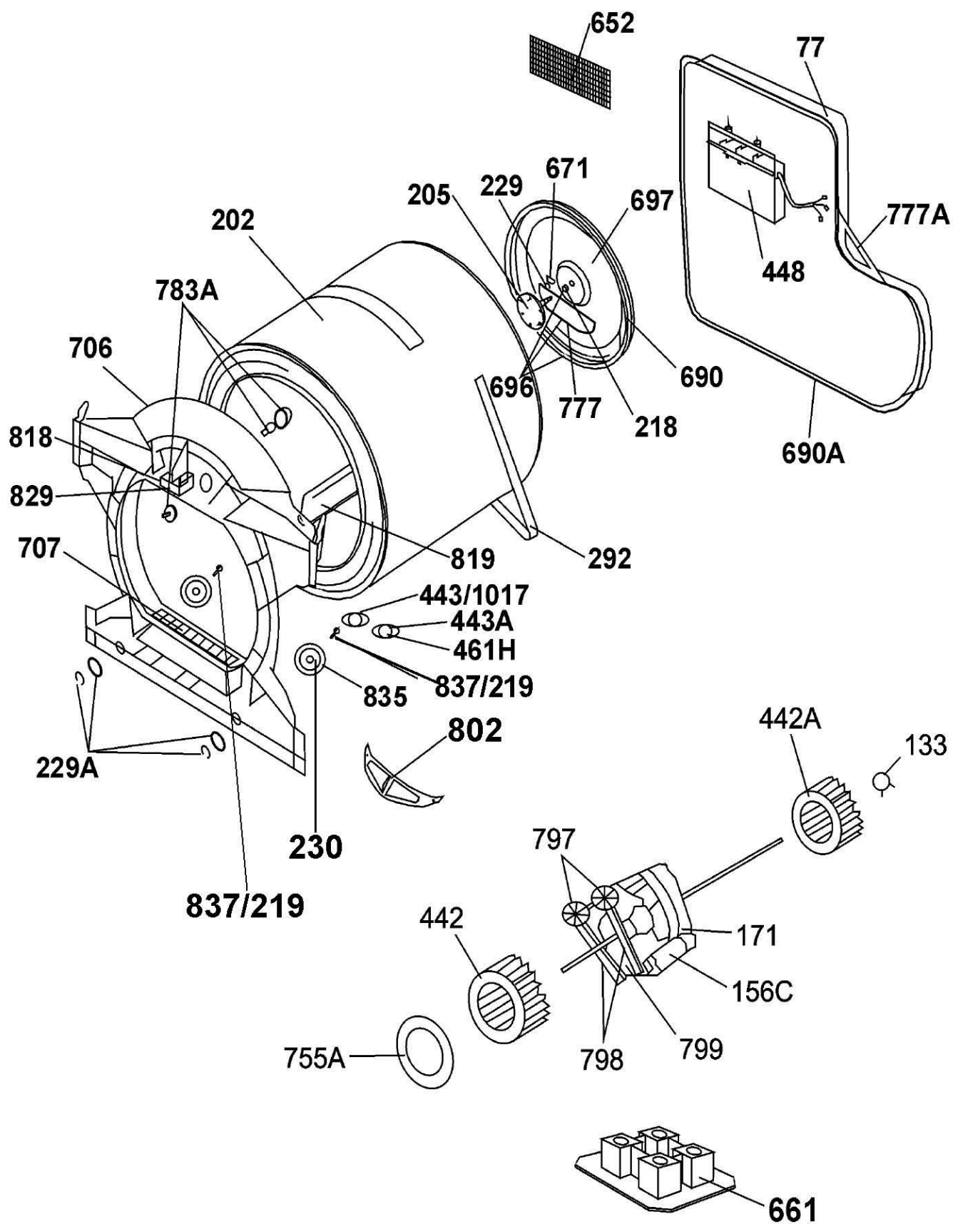
DRUM ASSY - CONDENSER EVC
