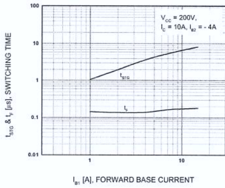
Figure 7. Resistive Load Switching Time
