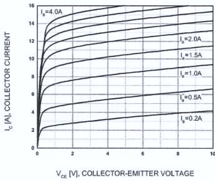
Figure 1. Static Characteristics
