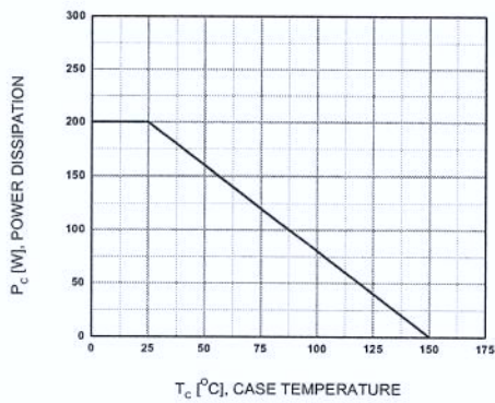
Figure 11. Power Derating
