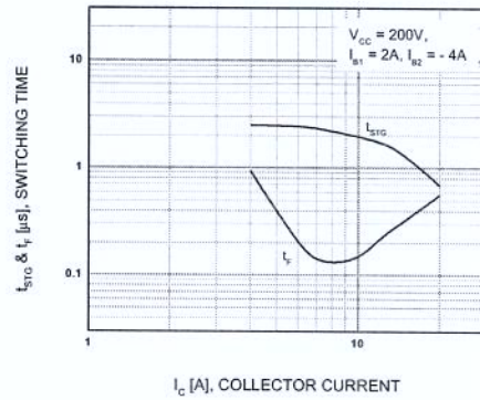
Figure 8. Resistive Load Switching Time
