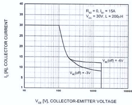
Figure 10. Reverse Bias Safe Operating Area
