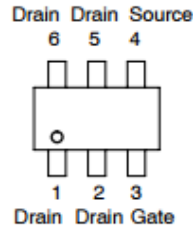
Figure 10: Pin description
