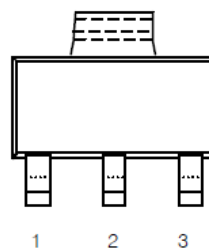
SOT-223 PKG (FRONT VIEW)
