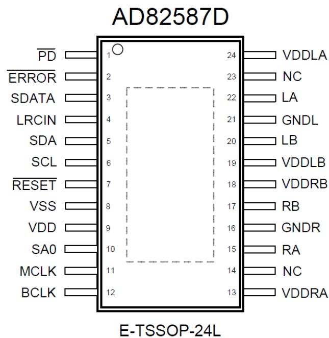
Figure 4: Pin description
