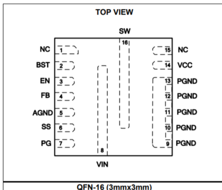
Figure 13: Pin Assignment
