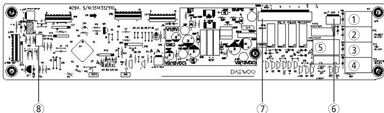
MAIN PCB
