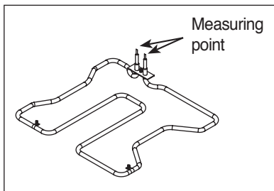
TOP HEATER
