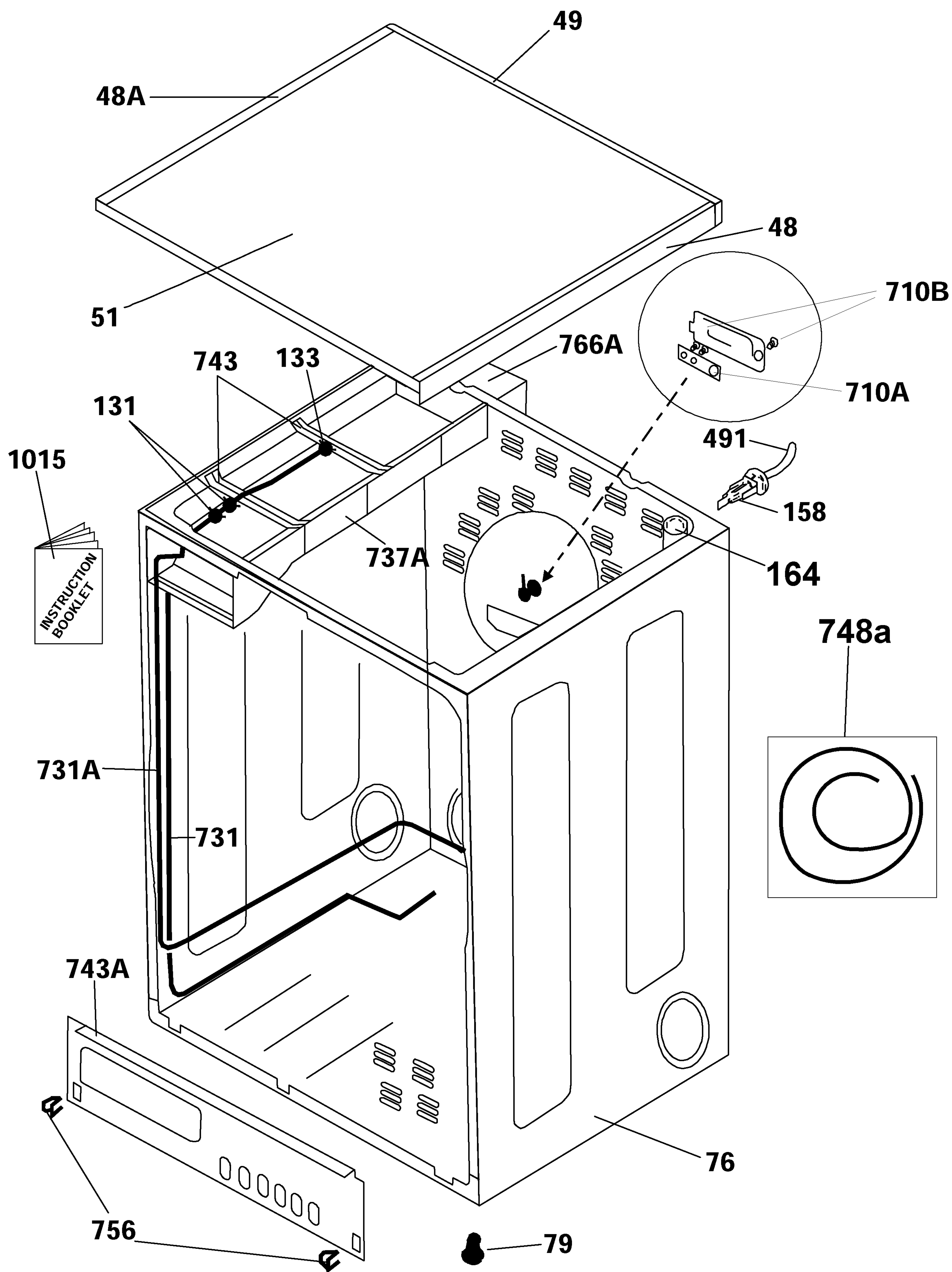
CONDENSER CABINET
