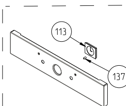
TOUCH CONTROLLED GLASS CONTROL PANEL ASSEMBLY (OPTIONAL)
