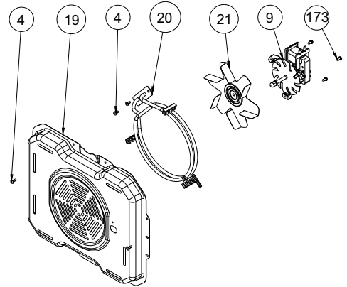
RING HEATING ELEMENT WITH FAN (OPTIONAL)
